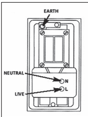
Wiring Diagram
